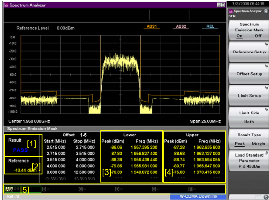
Figure 7.6-5 Display items for Measurement results
