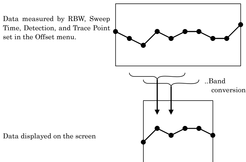
Figure 7.6-6 Band conversion (IBW)
