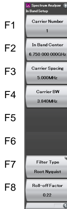
Figure 7.2-2 In Band Setup function menu
