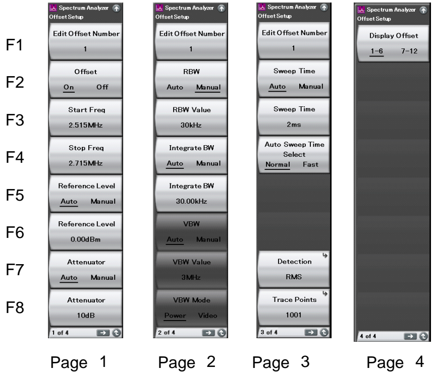
Figure 7.6-3 Offset Setup function menu
