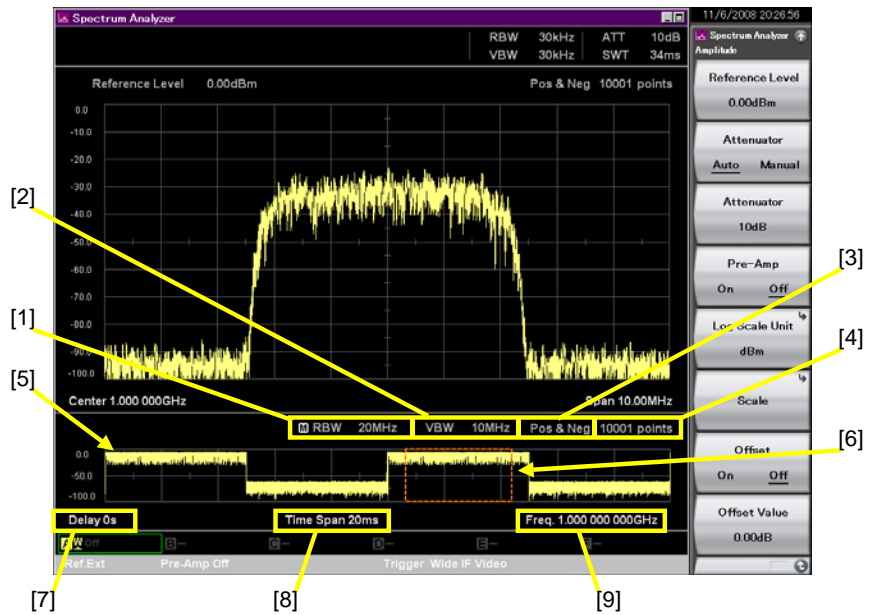
Figure 5.2.2-1 Gate View
